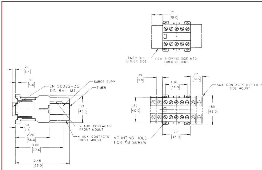
Open-Type, AC-Controlled Contactors and Control Relays, STD and Quick-Connect Terminal
